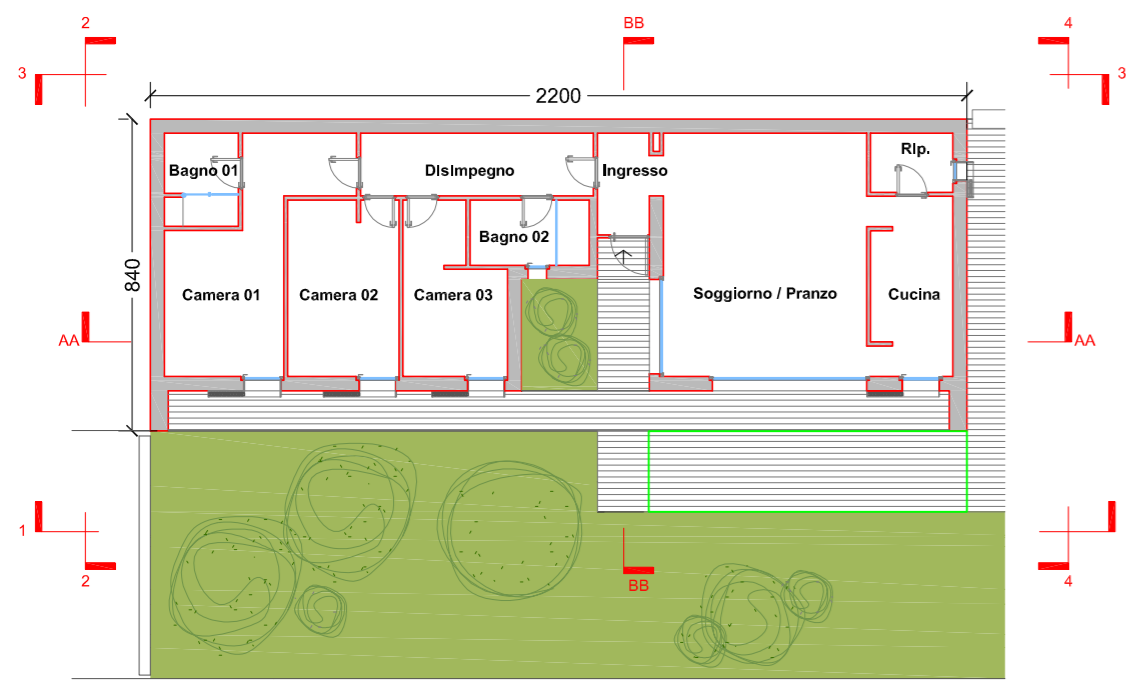
Piano terra 1 : 200
